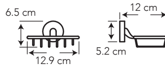
Jabonera COD. SG0016620161CW
